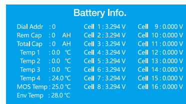
◆ On the Battery info page, the cell temperature, ambient temperature, and MOS temperature are displayed on the left, and the voltage values for each of the 16 cells are displayed on the right.
